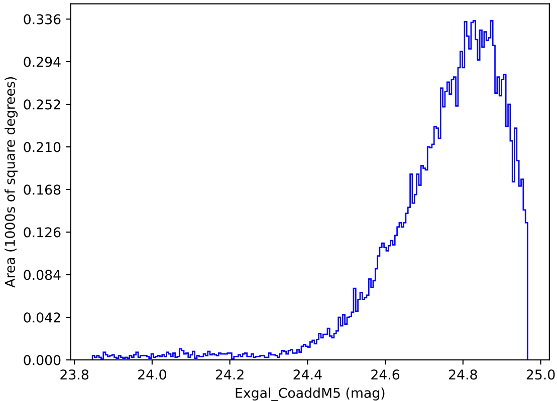
ddf_loaded_half_fl2_v3.4_10yrs WFD y band: Exgal_CoaddM5
