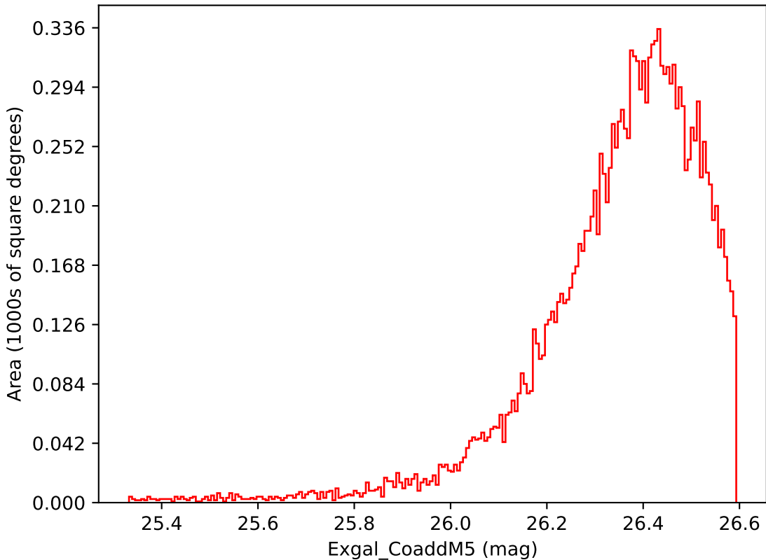
ddf_loaded_half_fl2_v3.4_10yrs WFD i band: Exgal_CoaddM5
