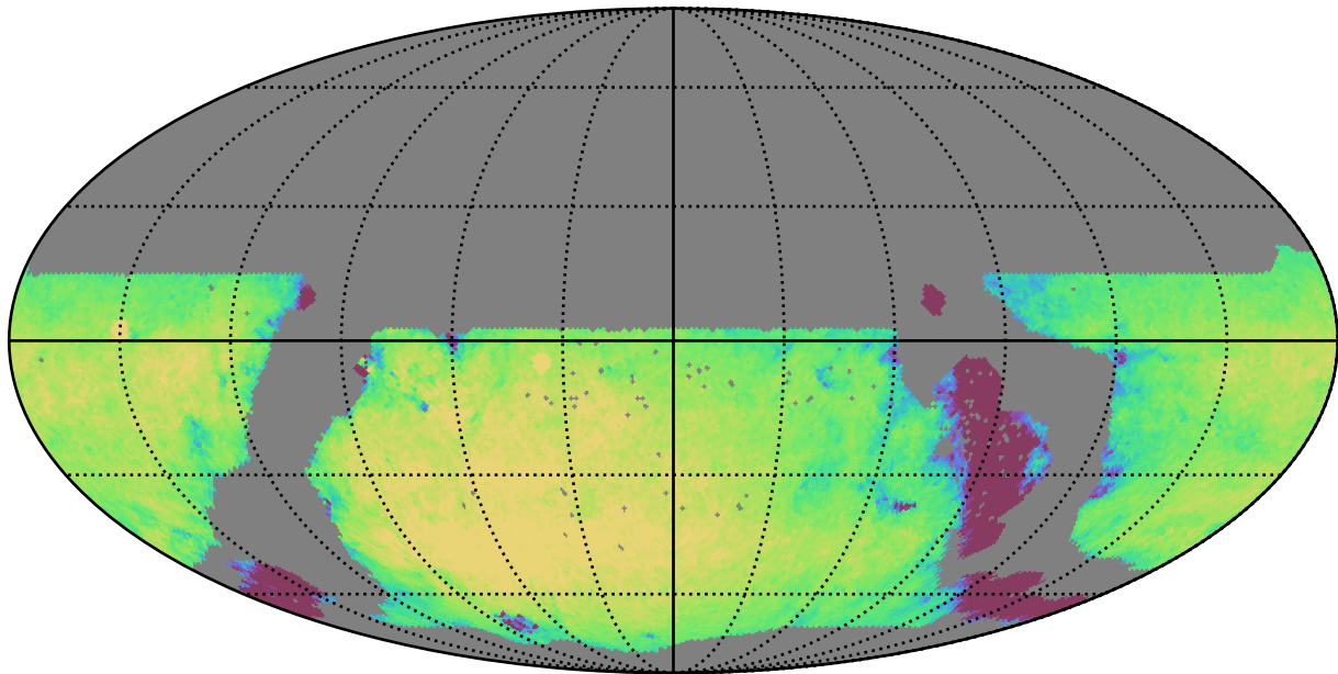
ddf_loaded_half_fl2_v3.4_10yrs WFD g band: Exgal_CoaddM5
