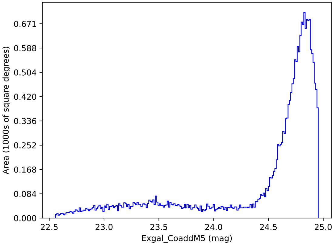
ddf_loaded_half_fl2_v3.4_10yrs All sky y band: Exgal_CoaddM5
