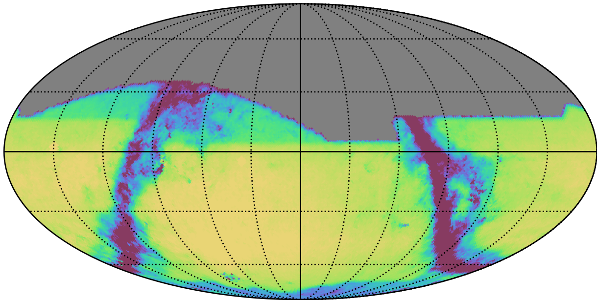
ddf_loaded_half_fl2_v3.4_10yrs All sky r band: Exgal_CoaddM5
