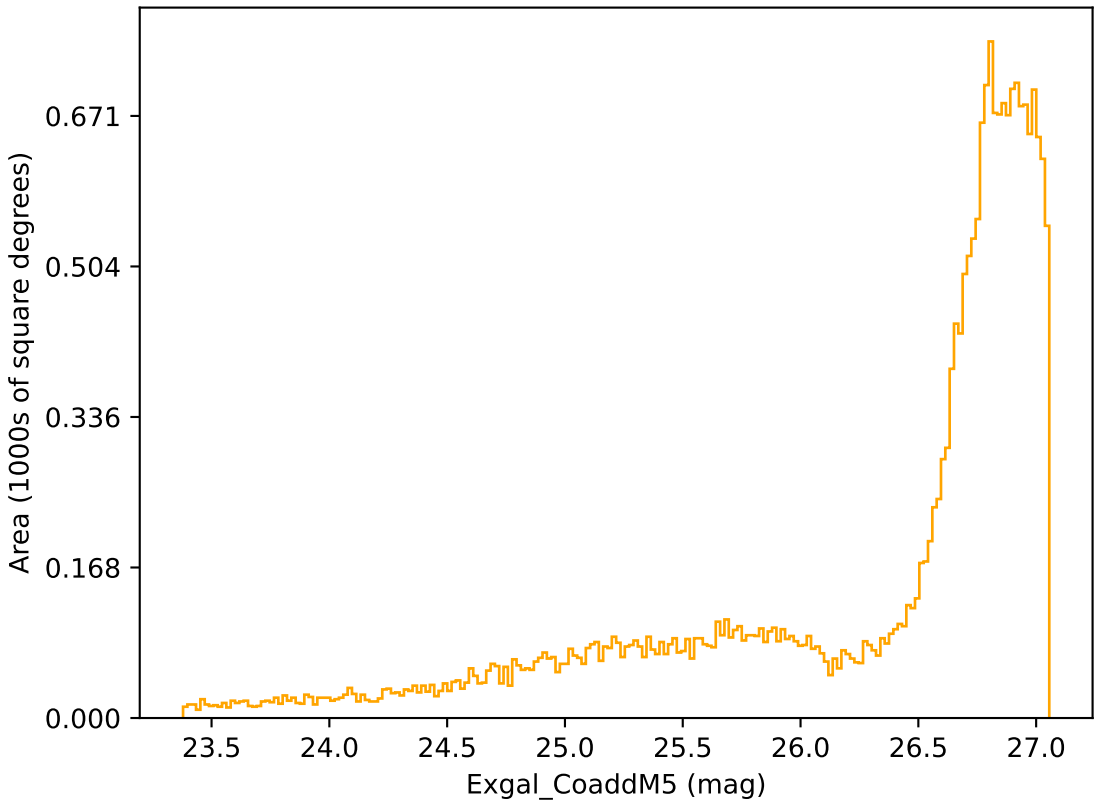
ddf_loaded_half_fl2_v3.4_10yrs All sky r band: Exgal_CoaddM5
