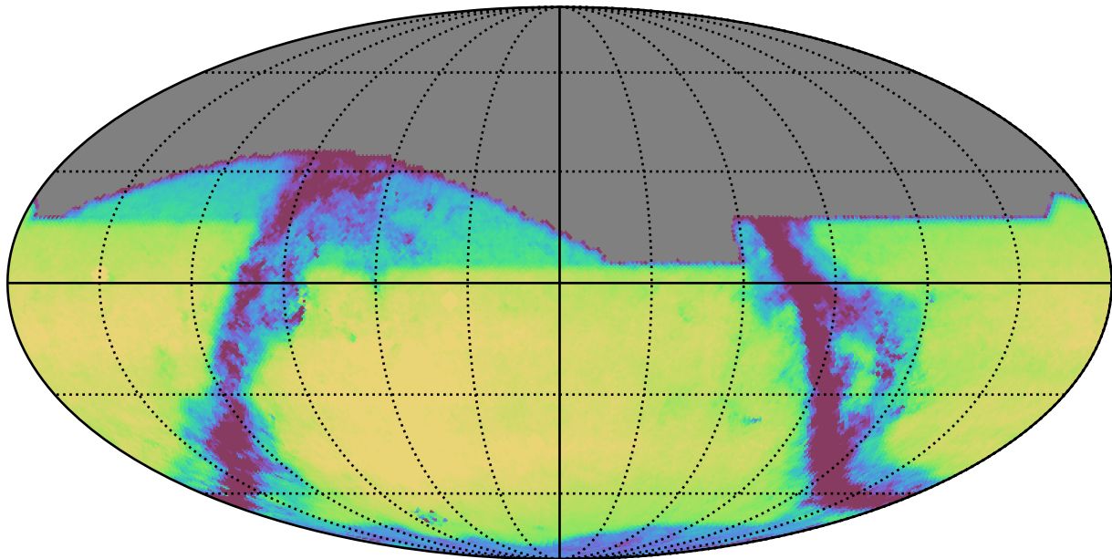
ddf_loaded_half_fl2_v3.4_10yrs All sky i band: Exgal_CoaddM5
