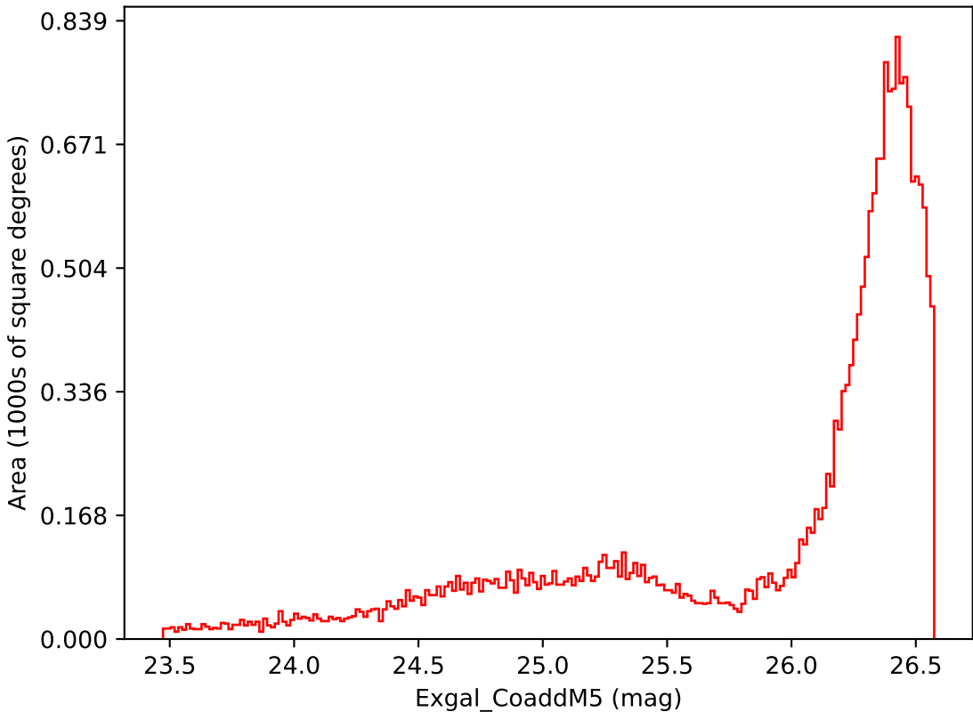
ddf_loaded_half_fl2_v3.4_10yrs All sky i band: Exgal_CoaddM5
