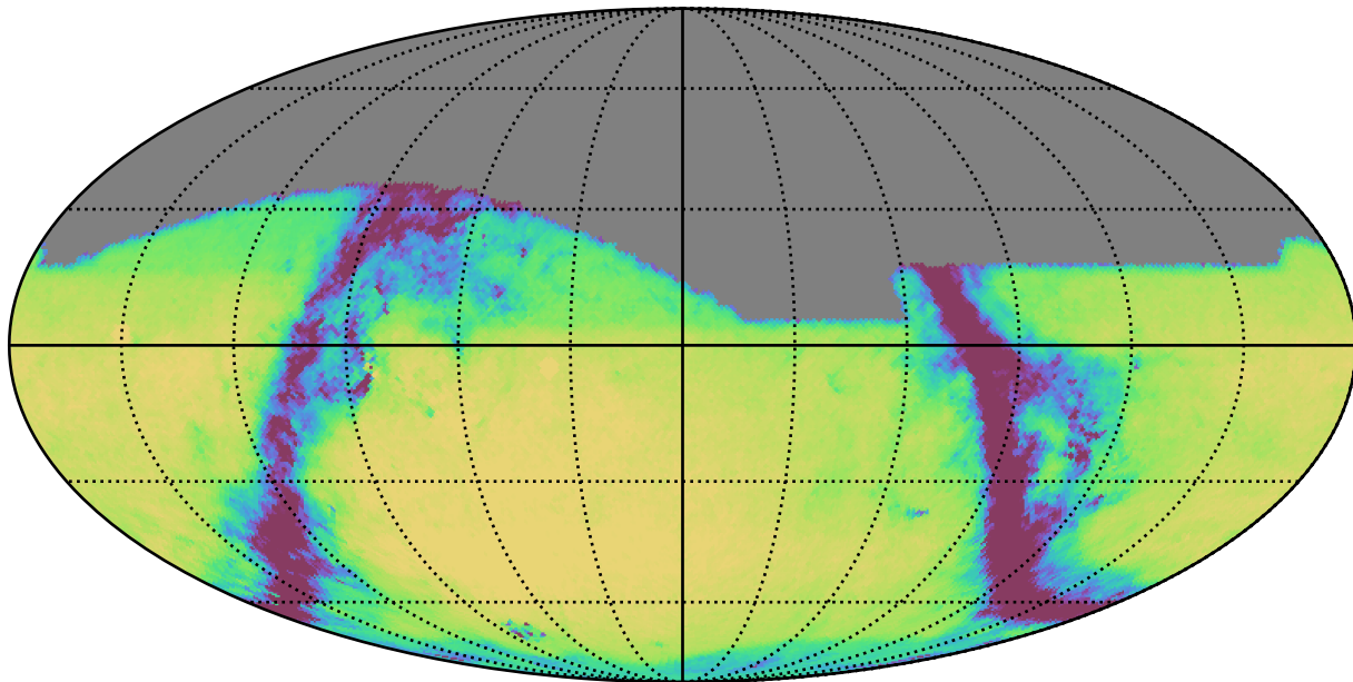
ddf_loaded_half_fl2_v3.4_10yrs All sky g band: Exgal_CoaddM5
