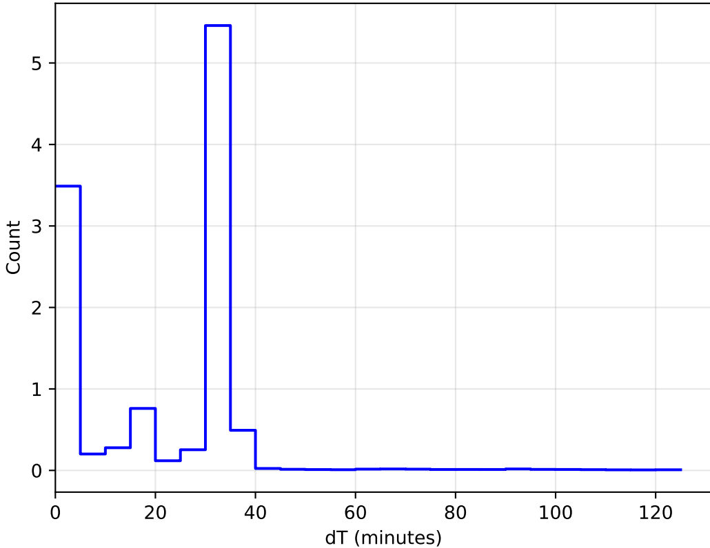
ddf_loaded_half_fl2_v3.4_10yrs WFD: DeltaT Histogram
