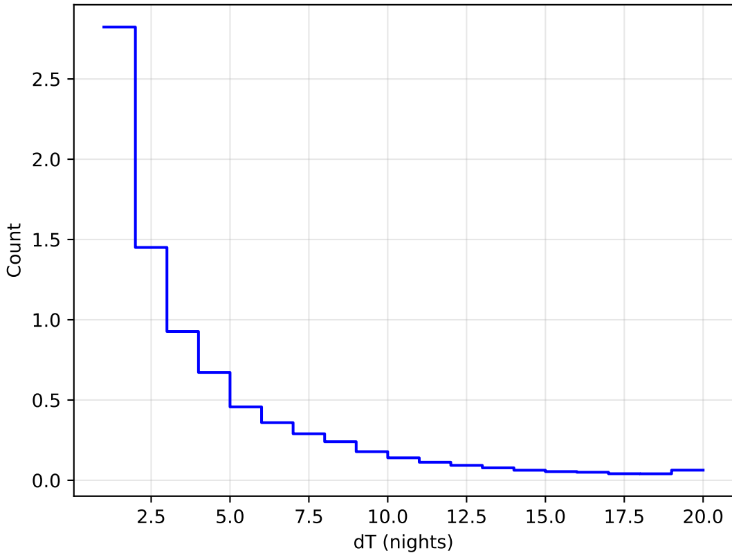
ddf_loaded_half_fl2_v3.4_10yrs WFD all bands: DeltaNight Histogram
