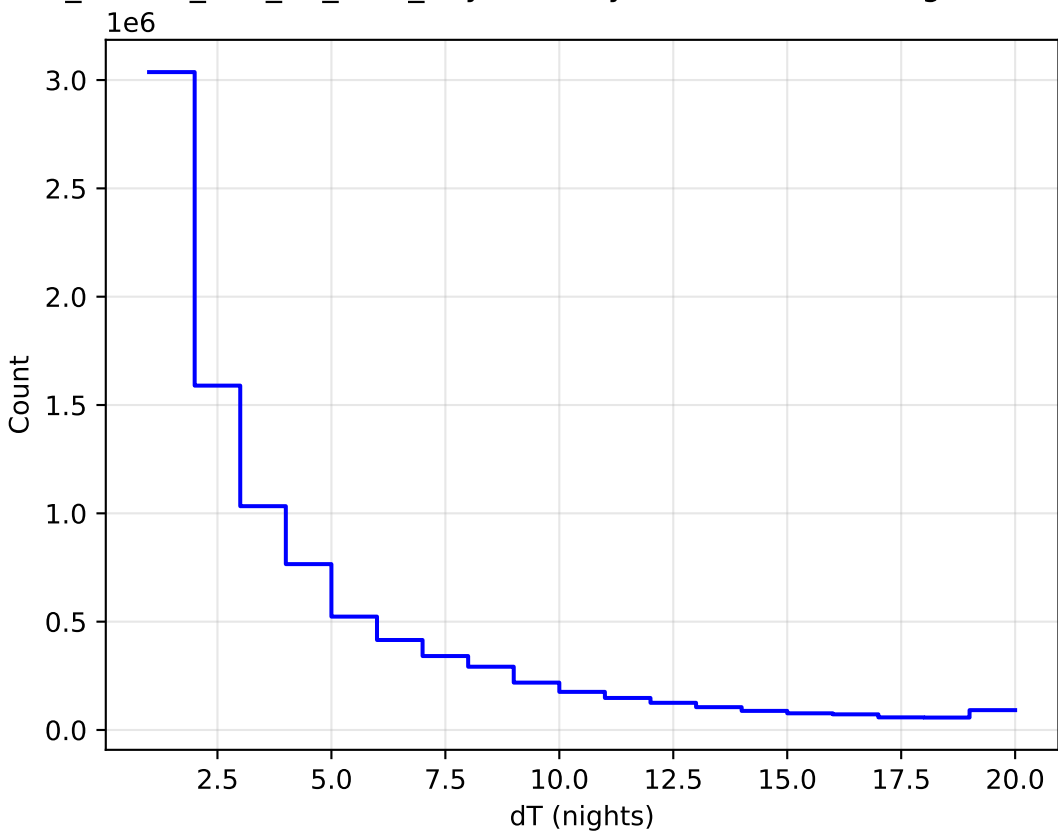
ddf_loaded_half_fl2_v3.4_10yrs All sky all bands: DeltaNight Histogram
