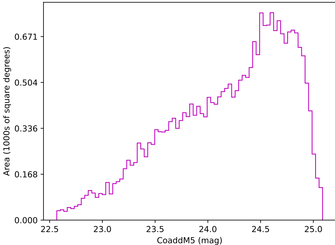
ddf_loaded_half_fl2_v3.4_10yrs Yr 3-4 z band: CoaddM5
