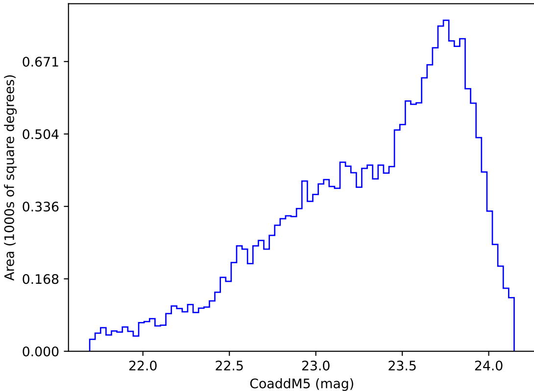
ddf_loaded_half_fl2_v3.4_10yrs Yr 3-4 y band: CoaddM5
