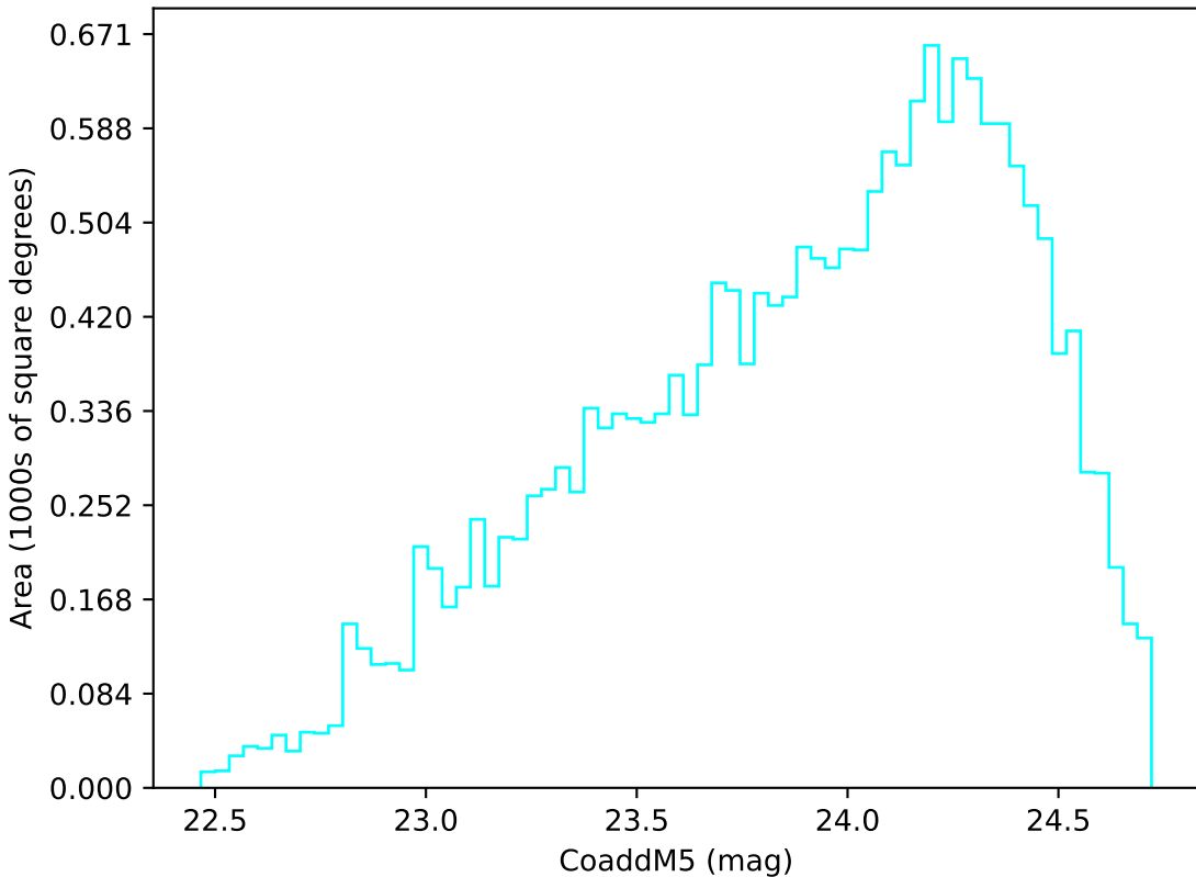
ddf_loaded_half_fl2_v3.4_10yrs Yr 3-4 u band: CoaddM5
