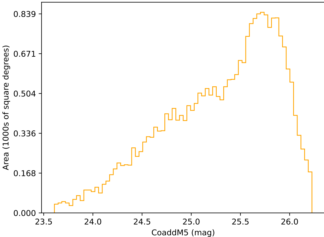
ddf_loaded_half_fl2_v3.4_10yrs Yr 3-4 r band: CoaddM5
