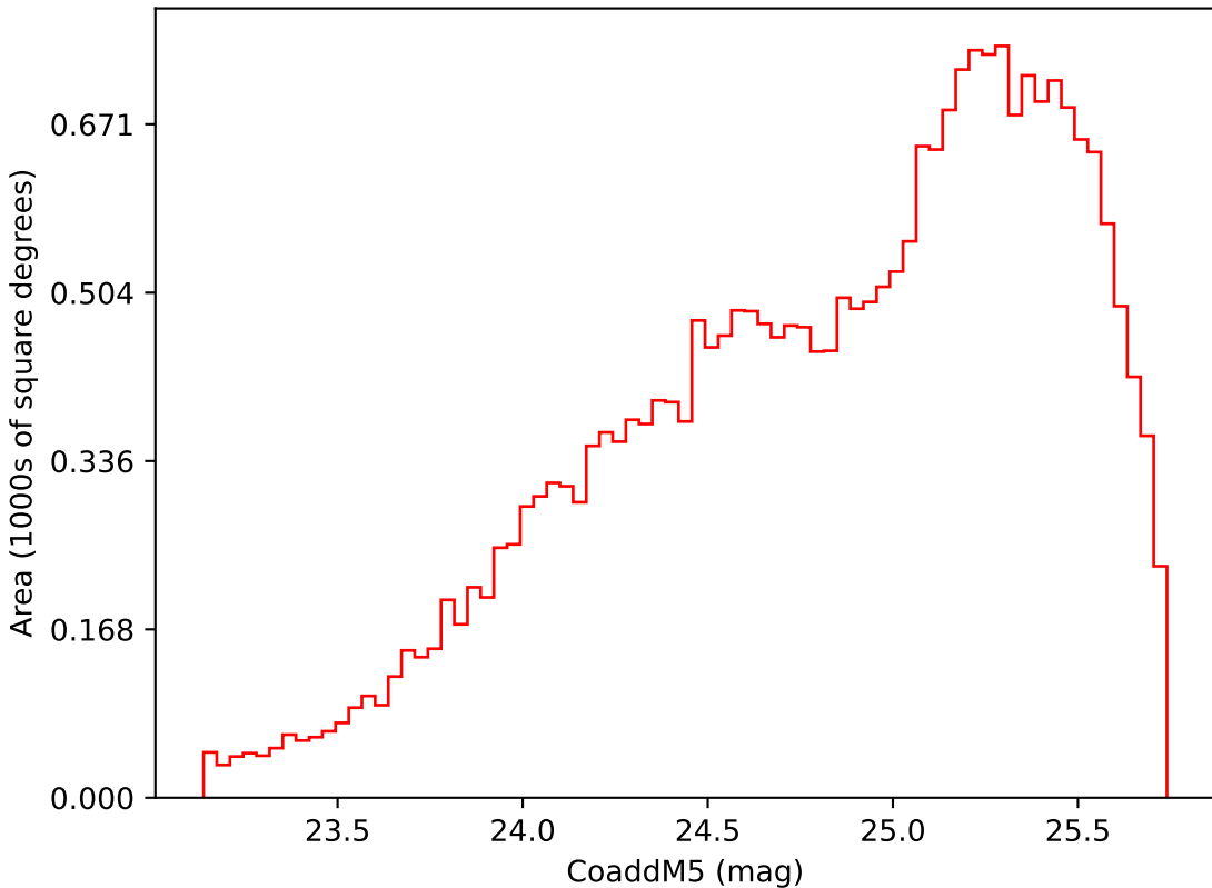
ddf_loaded_half_fl2_v3.4_10yrs Yr 3-4 i band: CoaddM5
