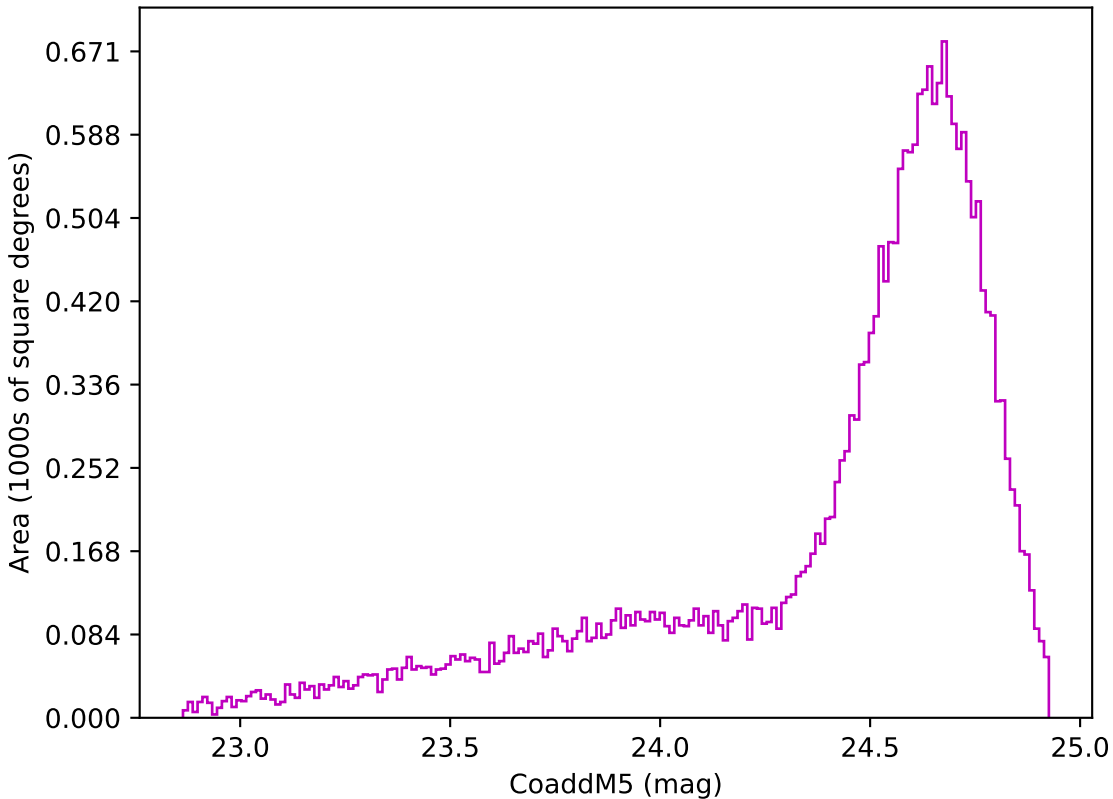
ddf_loaded_half_fl2_v3.4_10yrs Yr 1 z band: CoaddM5
