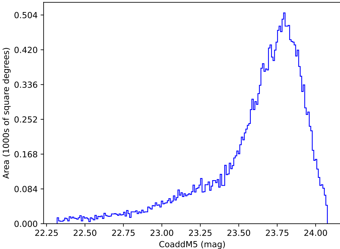
ddf_loaded_half_f12_v3.4_10yrs Yr 1 y band: CoaddM5
