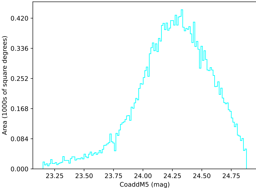
ddf_loaded_half_fl2_v3.4_10yrs Yr 1 u band: CoaddM5
