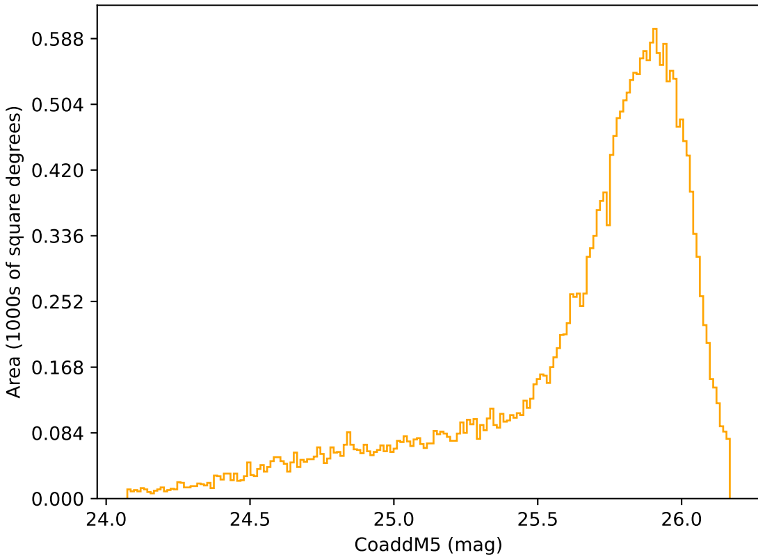
ddf_loaded_half_fl2_v3.4_10yrs Yr 1 r band: CoaddM5
