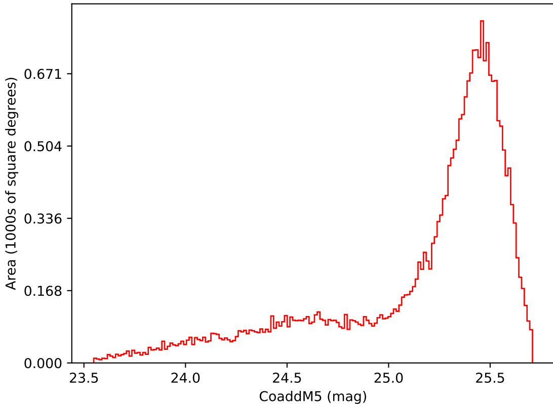
ddf_loaded_half_fl2_v3.4_10yrs Yr 1 i band: CoaddM5
