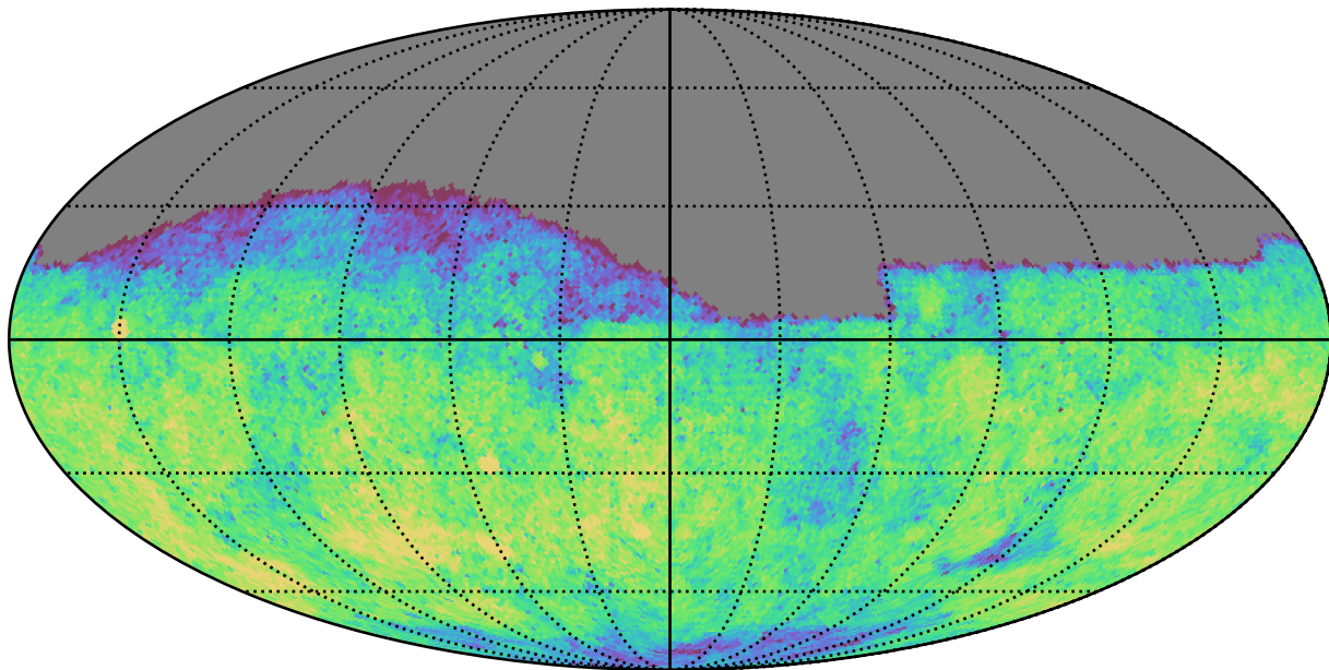
ddf_loaded_half_fl2_v3.4_10yrs Yr 1 g band: CoaddM5
