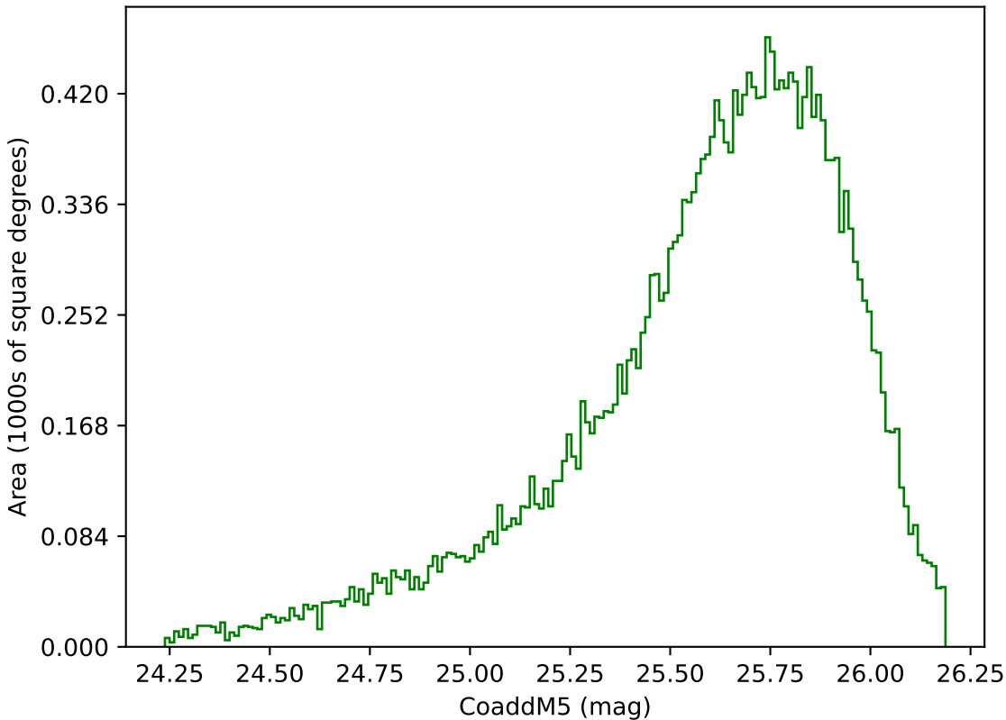
ddf_loaded_half_fl2_v3.4_10yrs Yr 1 g band: CoaddM5
