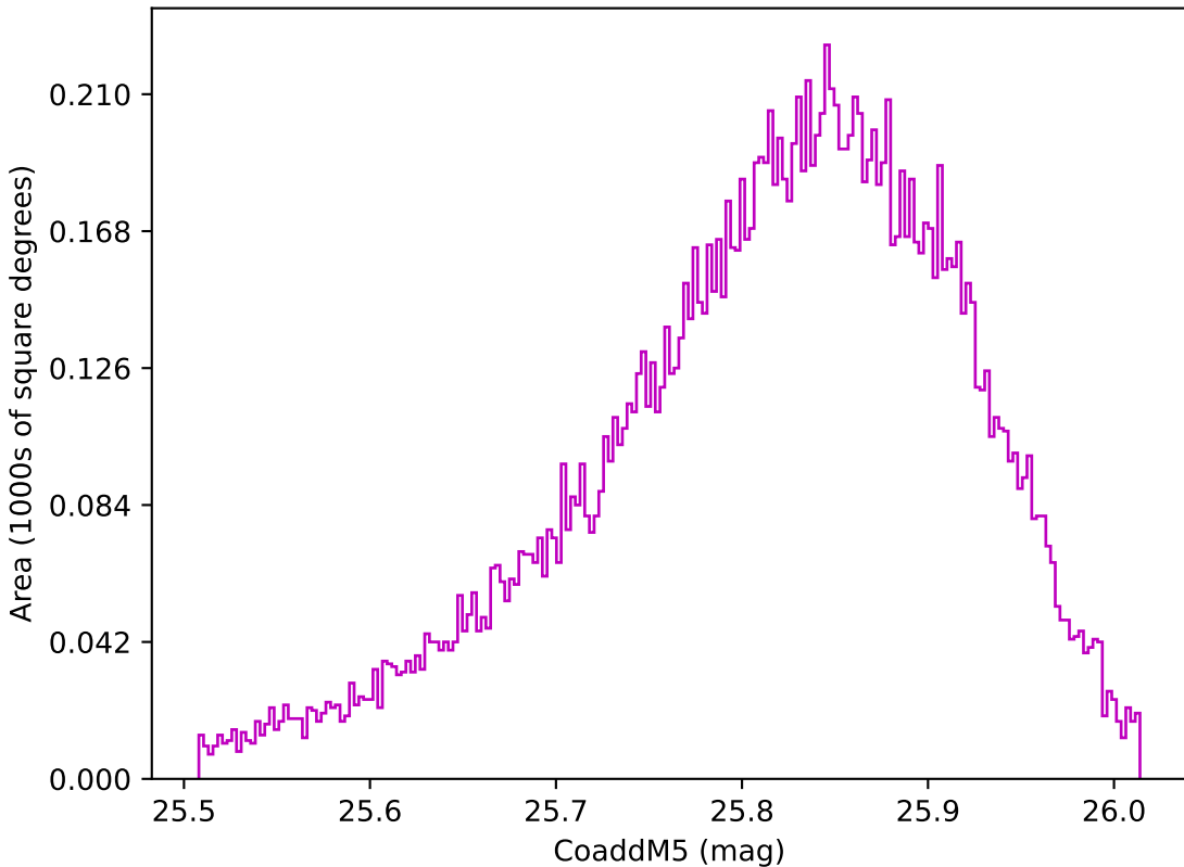
ddf_loaded_half_fl2_v3.4_10yrs WFD z band: CoaddM5
