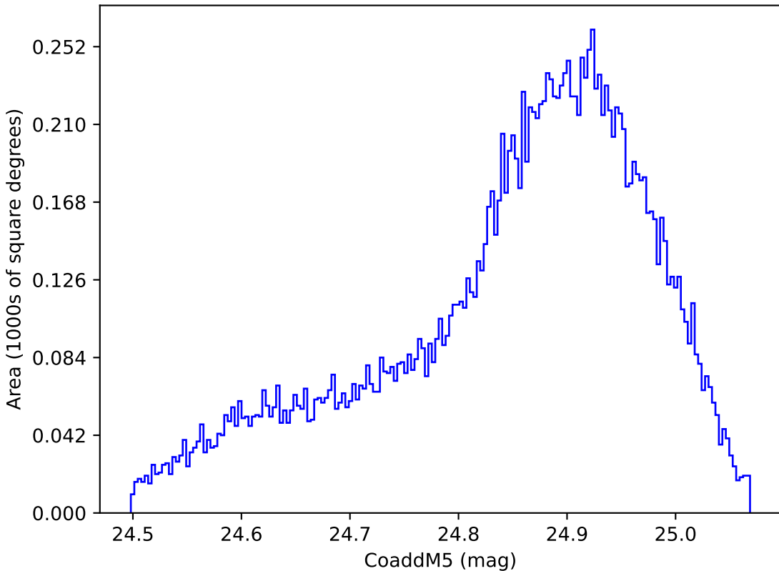
ddf_loaded_half_fl2_v3.4_10yrs WFD y band: CoaddM5
