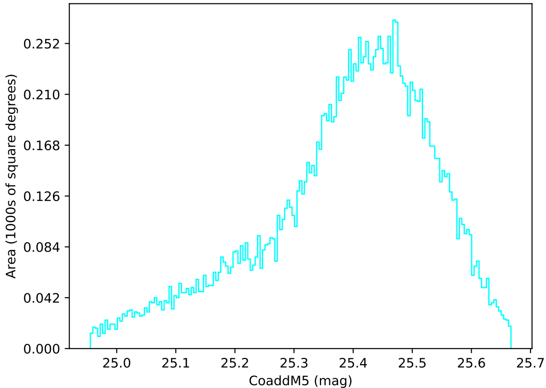
ddf_loaded_half_fl2_v3.4_10yrs WFD u band: CoaddM5
