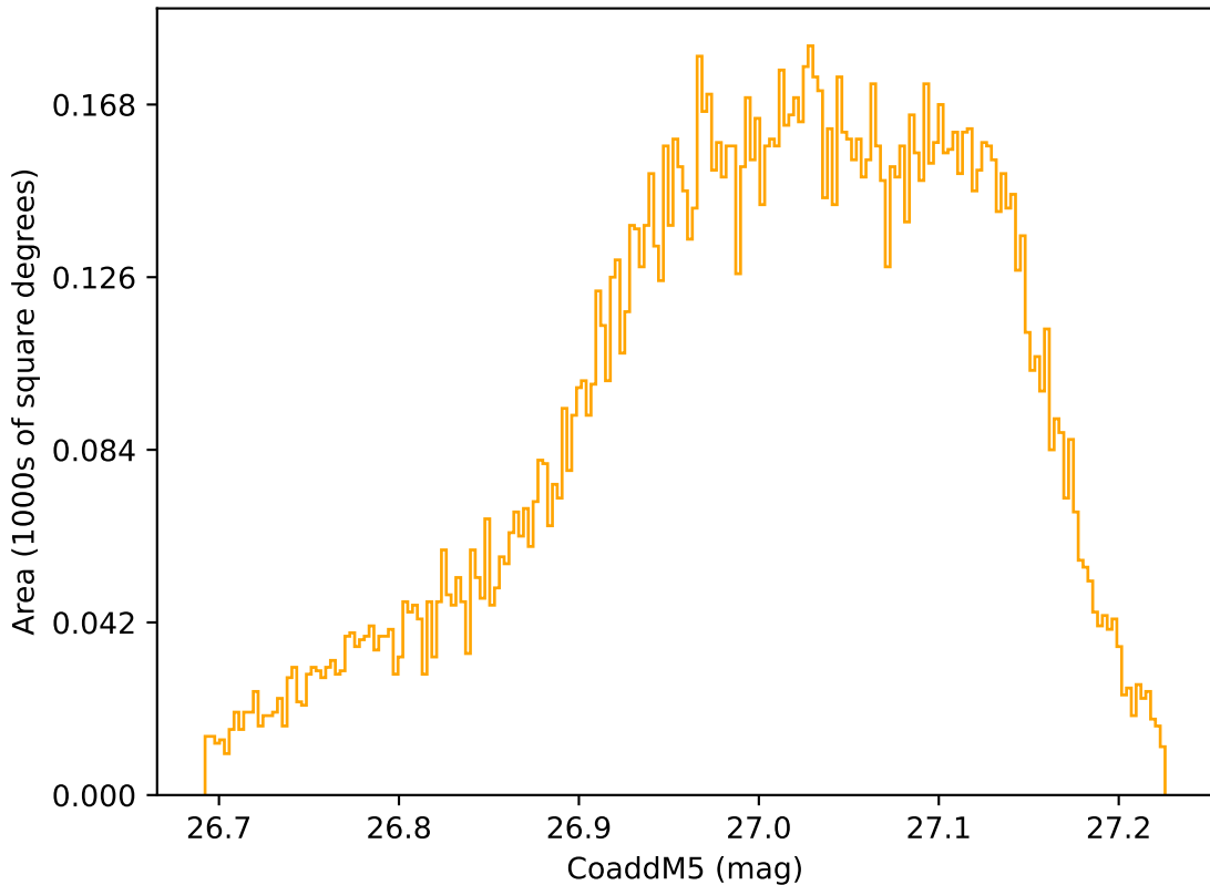
ddf_loaded_half_fl2_v3.4_10yrs WFD r band: CoaddM5
