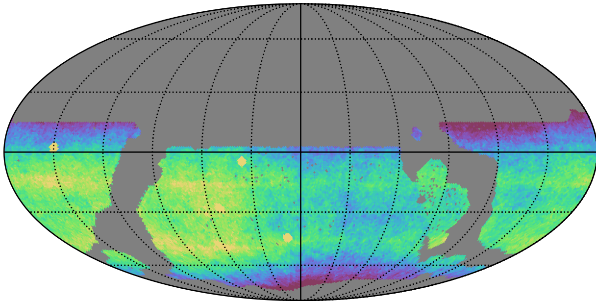
ddf_loaded_half_fl2_v3.4_10yrs WFD i band: CoaddM5
