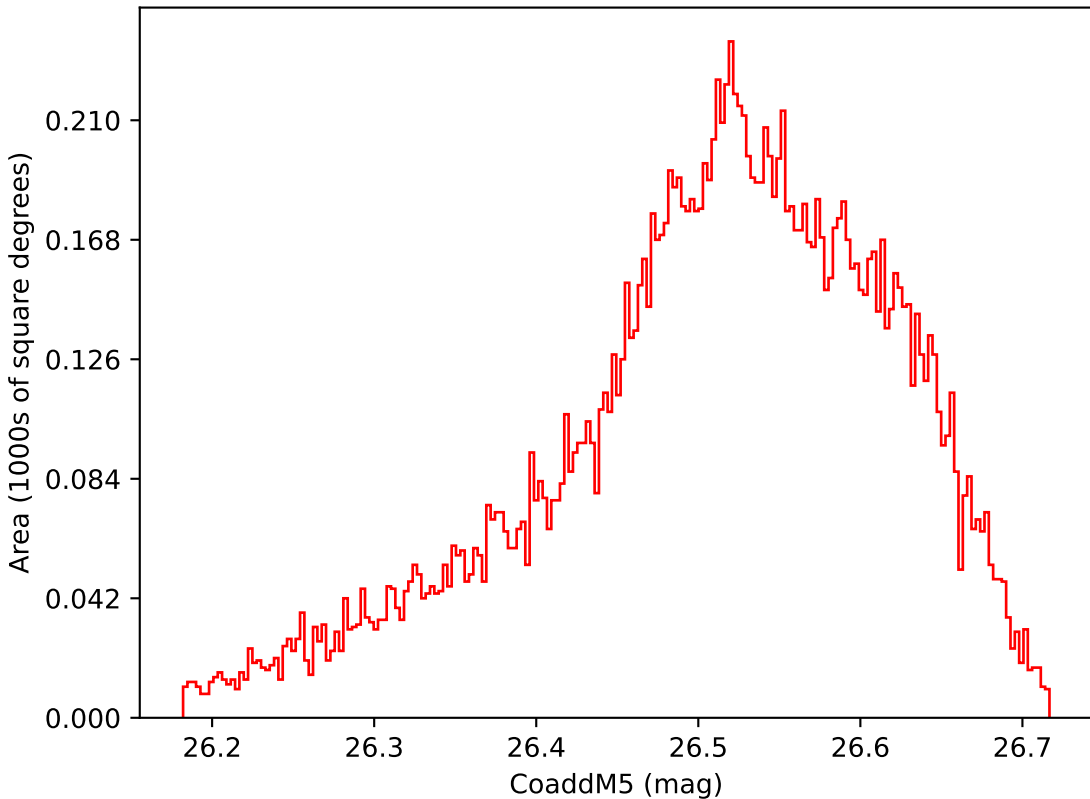
ddf_loaded_half_fl2_v3.4_10yrs WFD i band: CoaddM5
