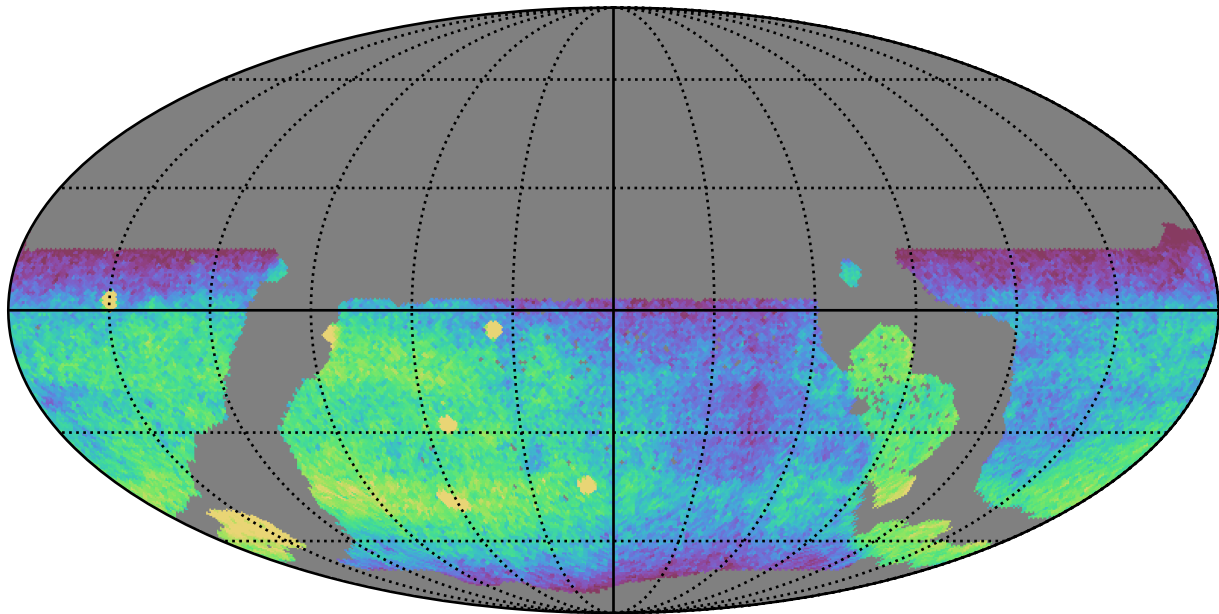
ddf_loaded_half_fl2_v3.4_10yrs WFD g band: CoaddM5
