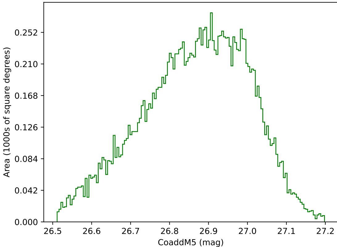
ddf_loaded_half_fl2_v3.4_10yrs WFD g band: CoaddM5
