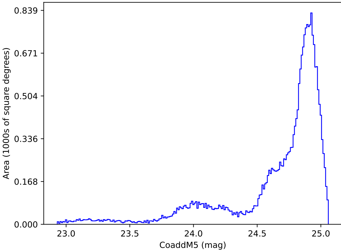
ddf_loaded_half_fl2_v3.4_10yrs All sky y band: CoaddM5
