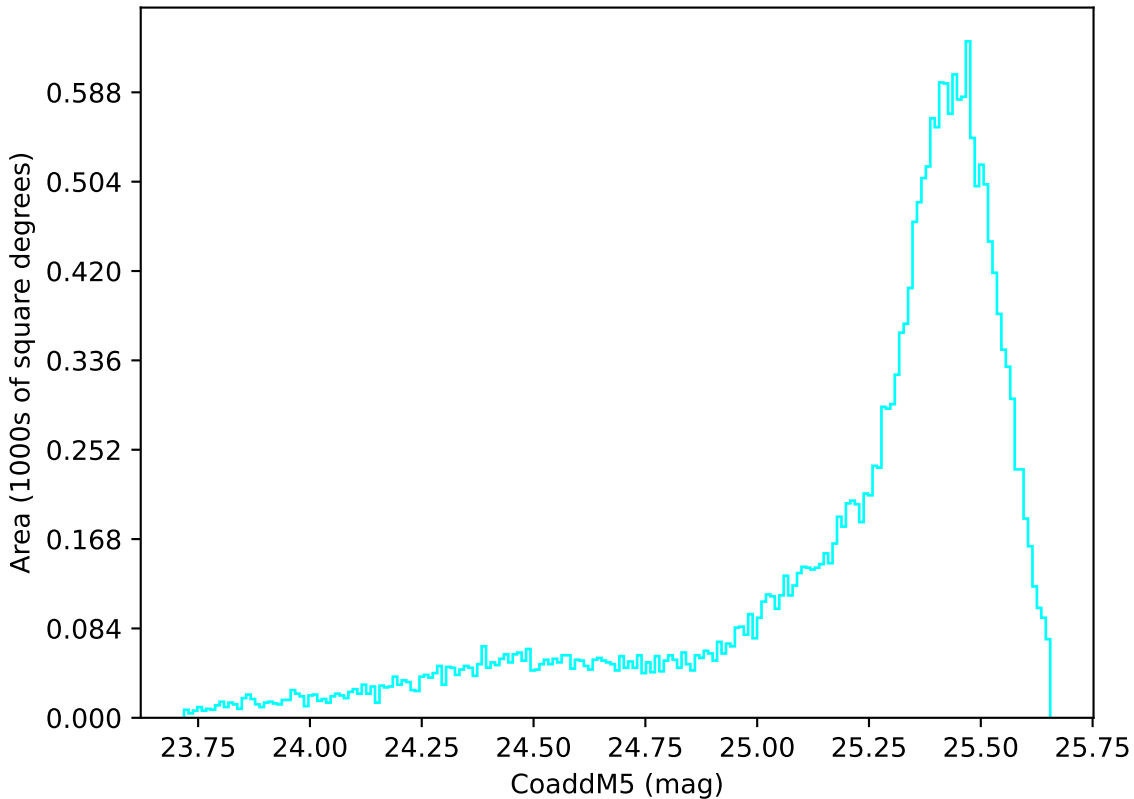
ddf_loaded_half_fl2_v3.4_10yrs All sky u band: CoaddM5
