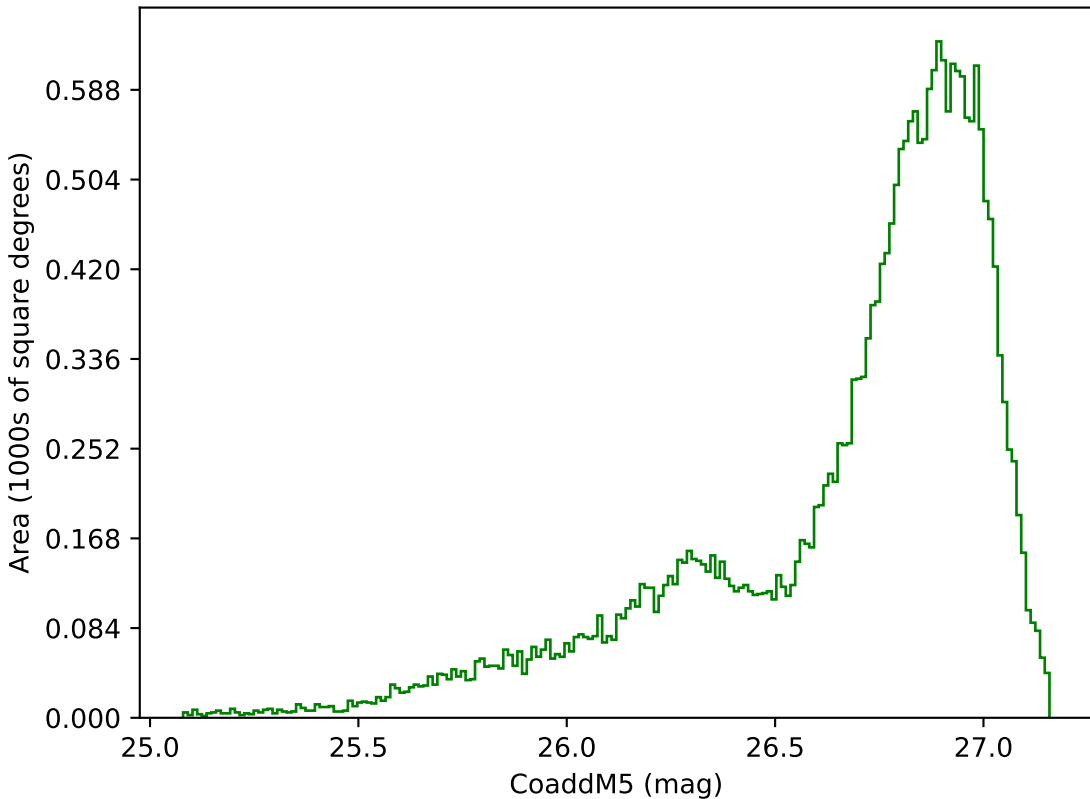
ddf_loaded_half_fl2_v3.4_10yrs All sky g band: CoaddM5
