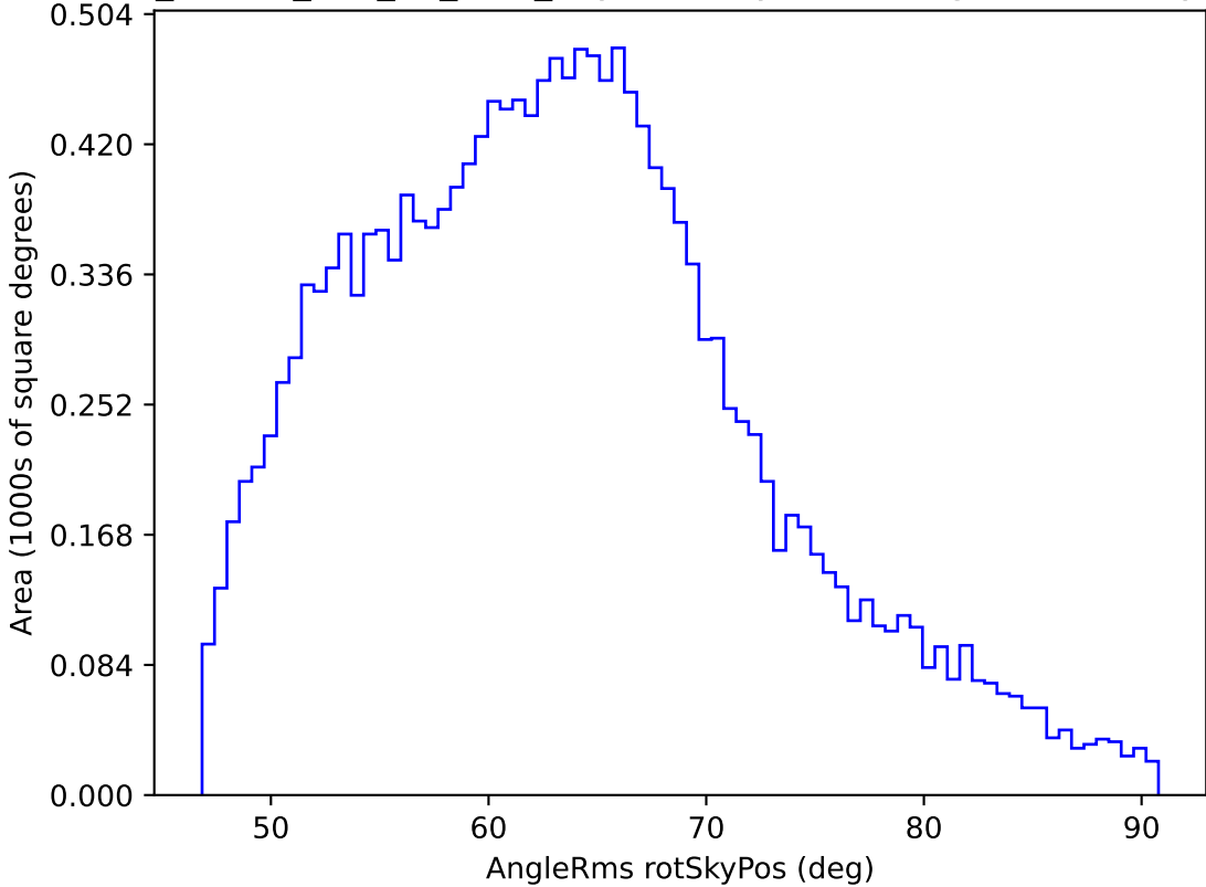
ddf_loaded_half_fl2_v3.4_10yrs WFD y band: AngleRms rotSkyPos
