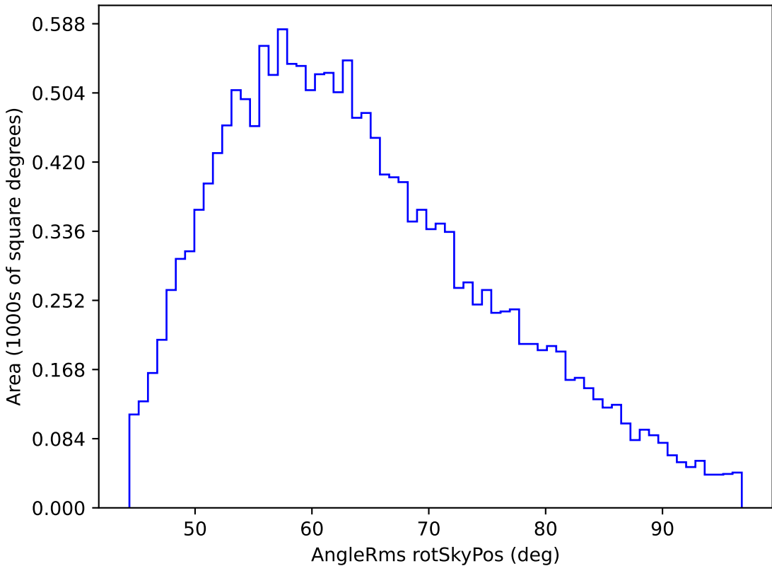
ddf_loaded_half_fl2_v3.4_10yrs WFD u band: AngleRms rotSkyPos
