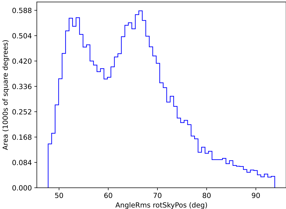
ddf_loaded_half_fl2_v3.4_10yrs WFD i band: AngleRms rotSkyPos
