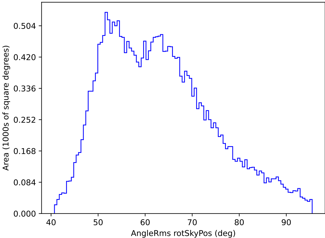
ddf_loaded_half_fl2_v3.4_10yrs All sky z band: AngleRms rotSkyPos
