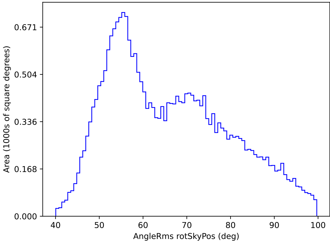
ddf_loaded_half_fl2_v3.4_10yrs All sky g band: AngleRms rotSkyPos
