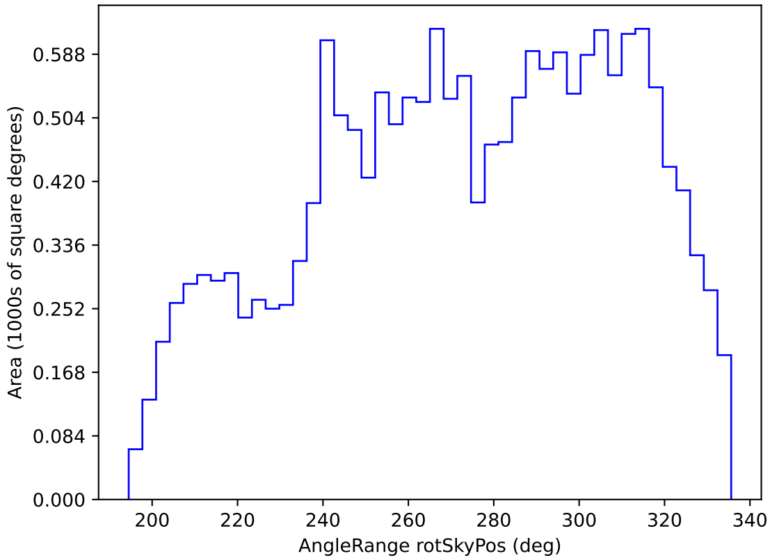
ddf_loaded_half_fl2_v3.4_10yrs WFD y band: AngleRange rotSkyPos
