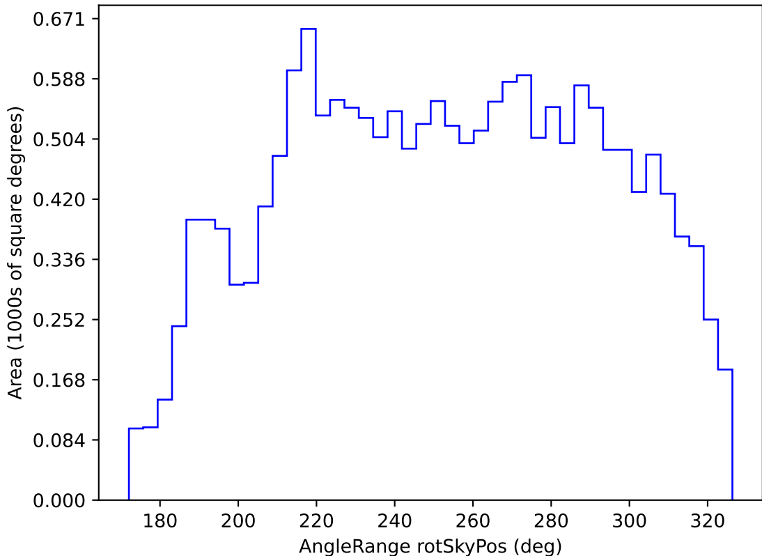
ddf_loaded_half_fl2_v3.4_10yrs WFD u band: AngleRange rotSkyPos
