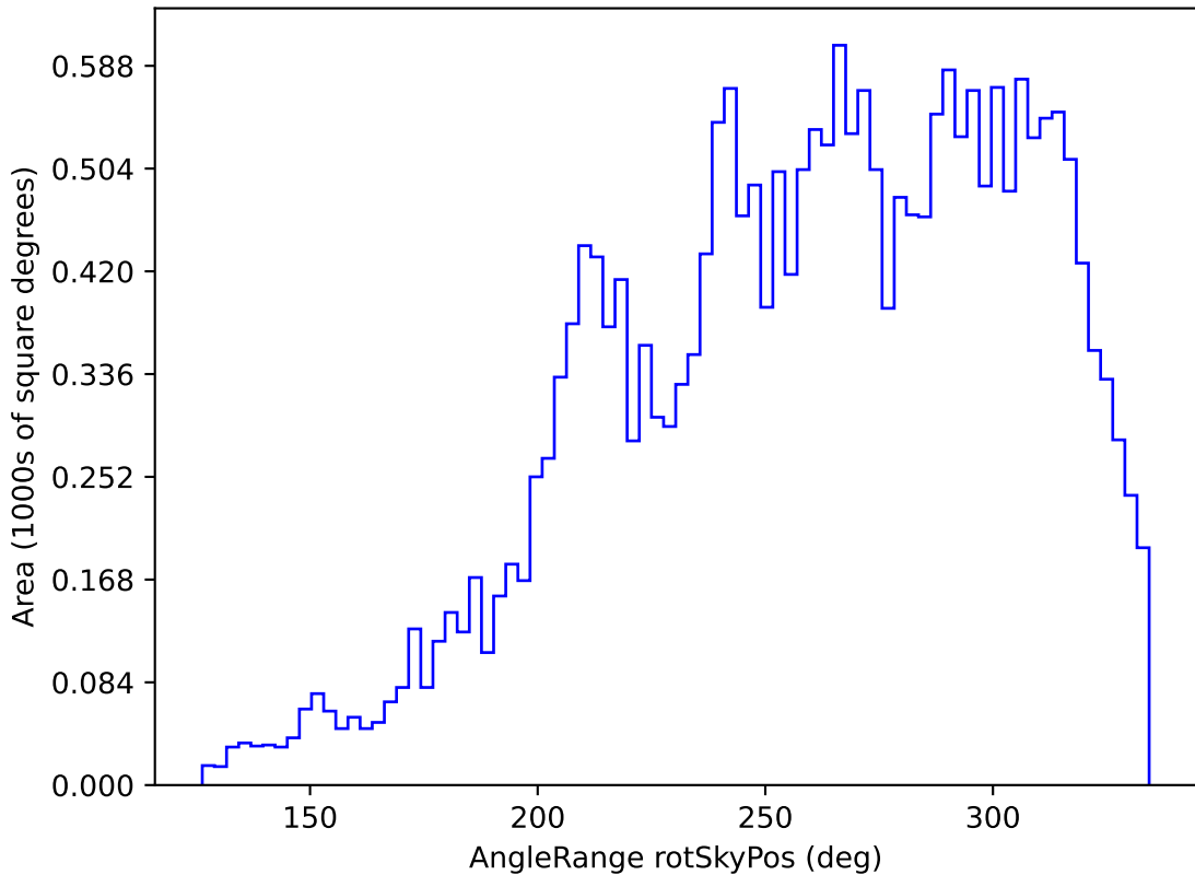
ddf_loaded_half_fl2_v3.4_10yrs All sky y band: AngleRange rotSkyPos
