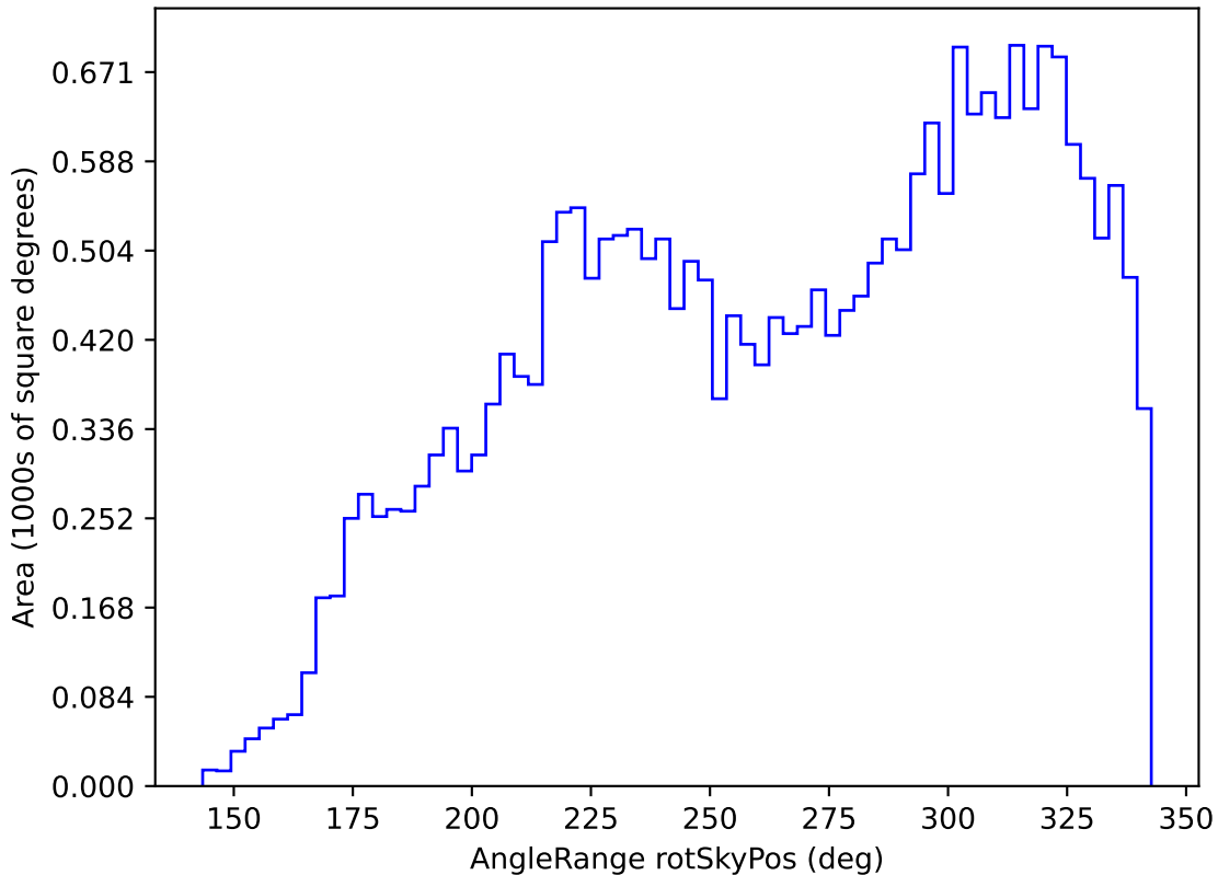
ddf_loaded_half_fl2_v3.4_10yrs All sky i band: AngleRange rotSkyPos
