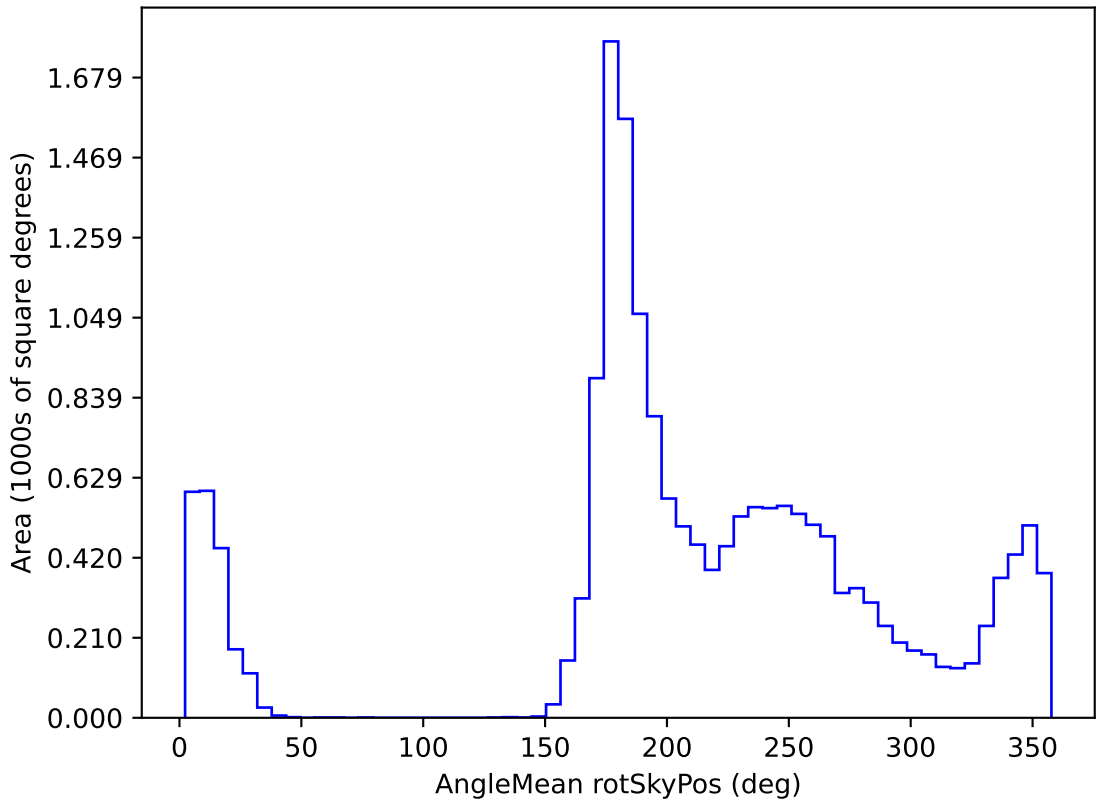
ddf_loaded_half_fl2_v3.4_10yrs WFD z band: AngleMean rotSkyPos
