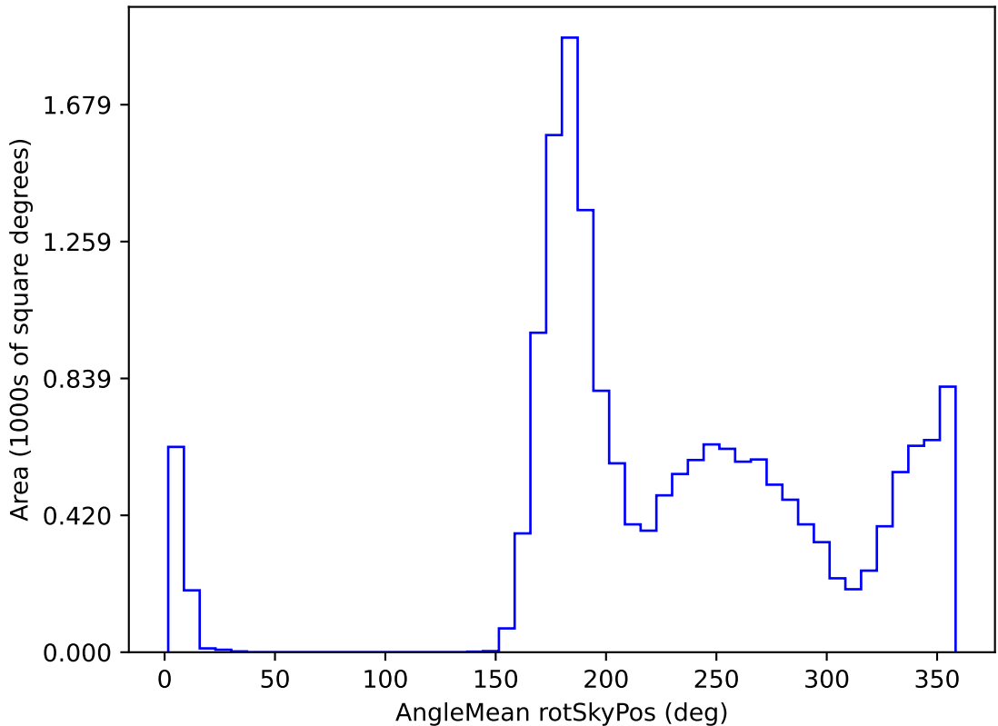
ddf_loaded_half_fl2_v3.4_10yrs WFD y band: AngleMean rotSkyPos
