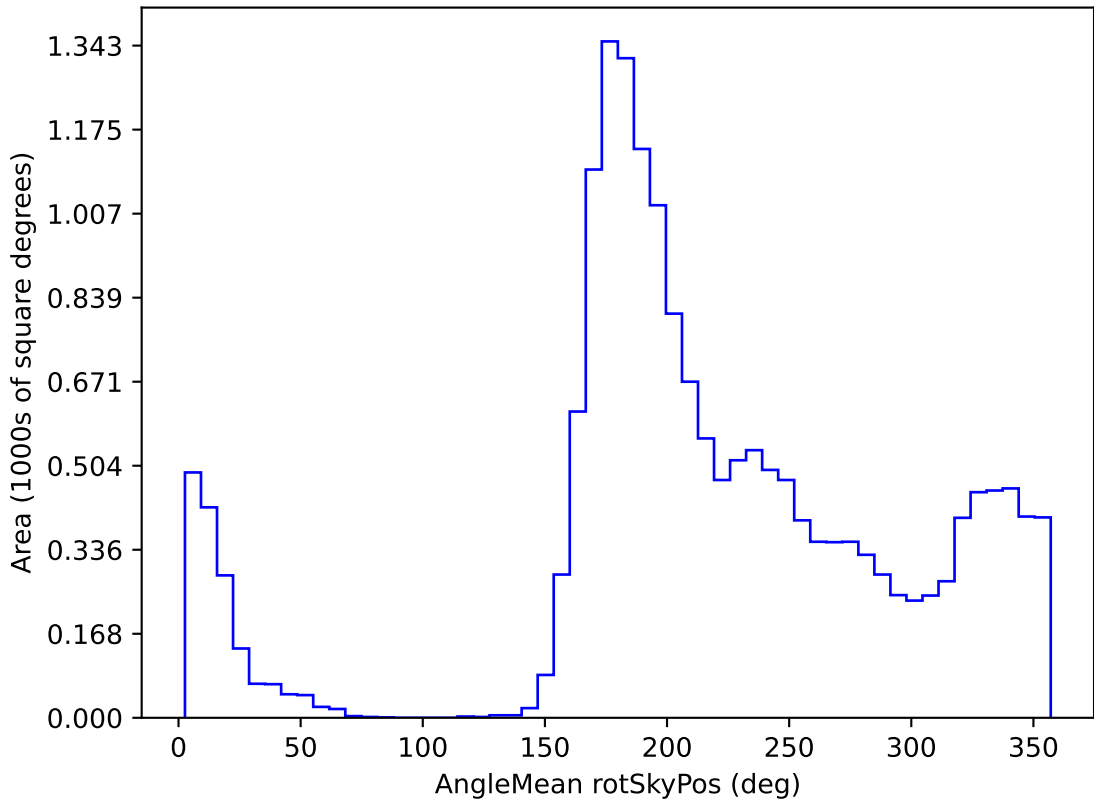
ddf_loaded_half_fl2_v3.4_10yrs WFD u band: AngleMean rotSkyPos
