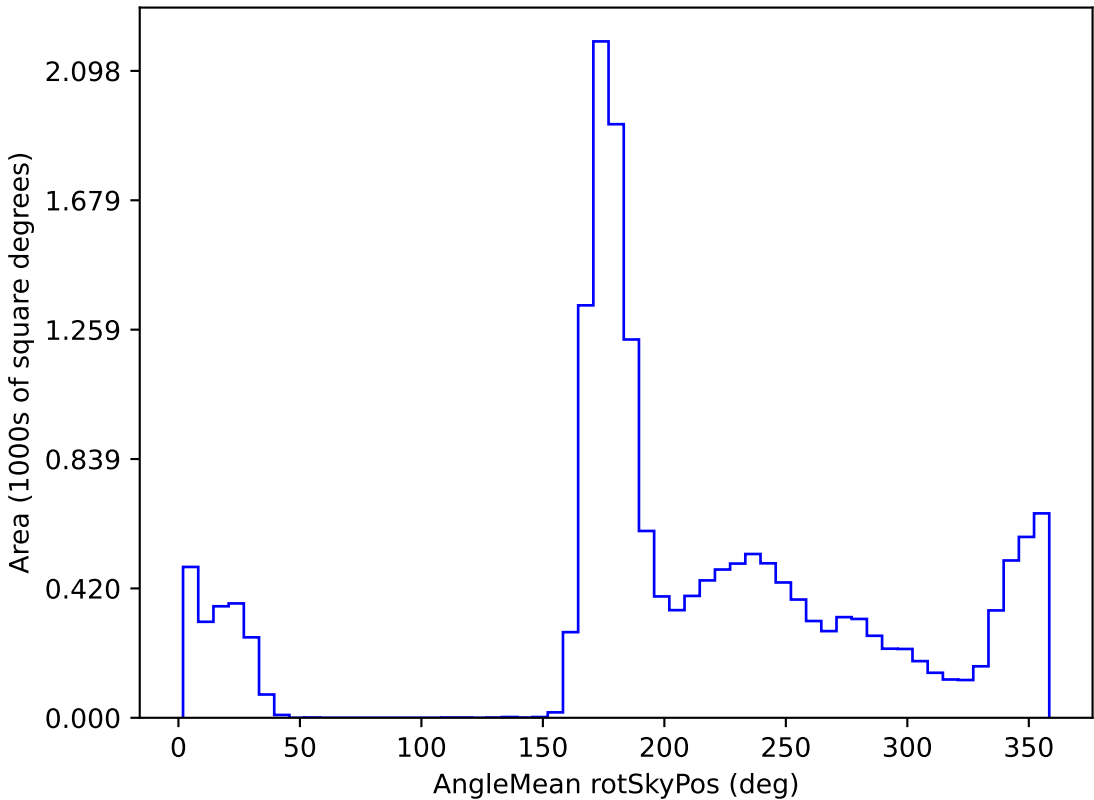
ddf_loaded_half_fl2_v3.4_10yrs WFD r band: AngleMean rotSkyPos
