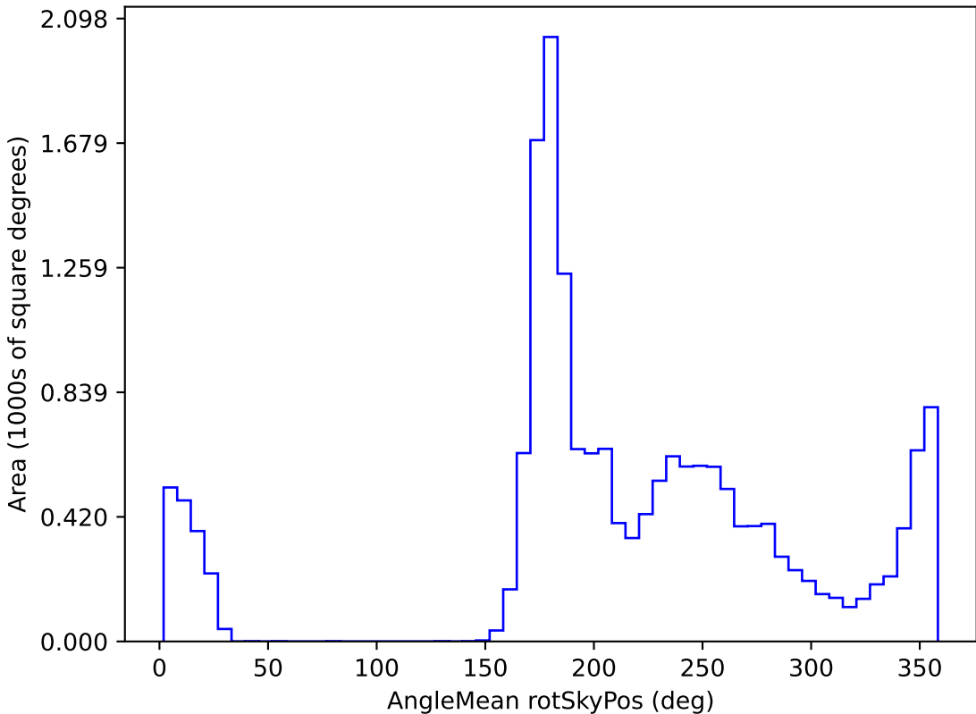
ddf_loaded_half_fl2_v3.4_10yrs WFD i band: AngleMean rotSkyPos
