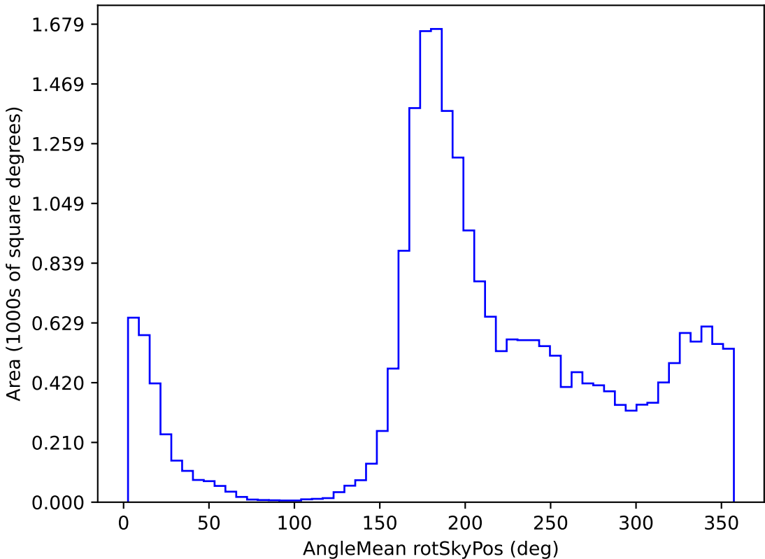
ddf_loaded_half_fl2_v3.4_10yrs All sky u band: AngleMean rotSkyPos
